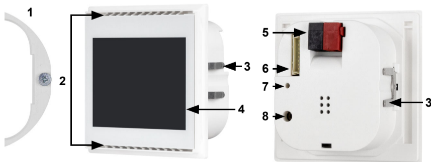
Fig. 1 1 Mounting adapter with screws 2 Openings for air circulation 3 Catches 4 Touch Display 5 KNX-terminal BUS +/- 6 Slot for connecting cable 7 Programming-LED (recessed) 8 Programming-Button (recessed) for teaching device
