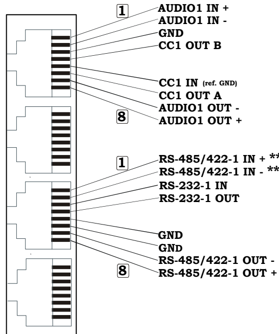
Figure 4. Socket pin assignments. The second port (A2/CC2) is similar in layout to port A1/CC1/ while the bottom port (D3/D4) is similar to the third (D1/D2). Input connector pins marked ** is the Input and Output for RS-485 2W operation (see text).
