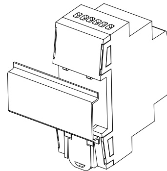
Figure 2: Mounting RailQUAD 8 on DIN rail
