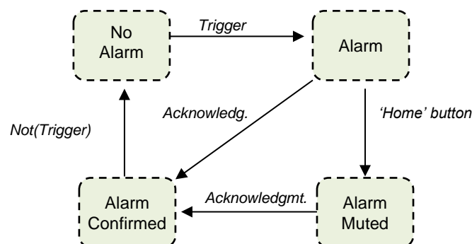
Figure 84. Alarm state diagram (case of confirmation previous to the alarm end).
