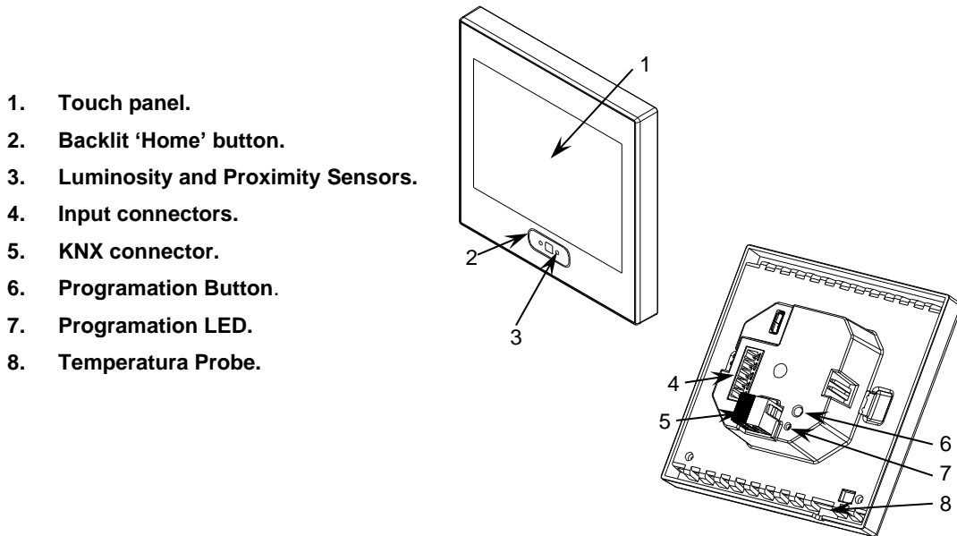
Figure 1. Schematic diagram Z35.
