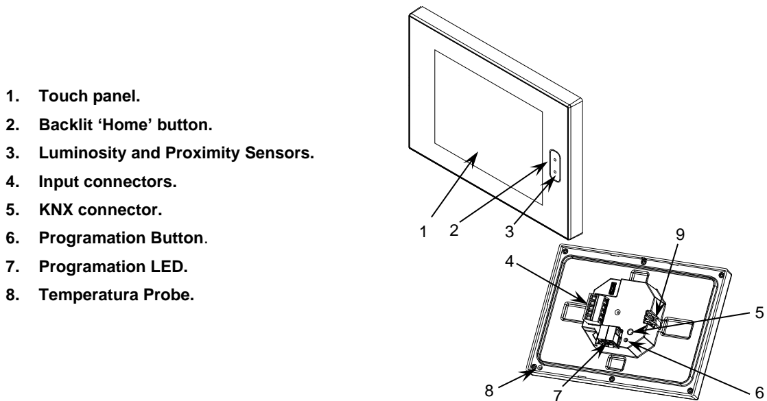
Figure 2. Schematic diagram Z40.
