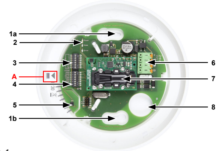
Fig. 1 1 a + b Long holes for mounting (hole distance 60mm) 2 LEDs: Green Power/Operating voltage. Red Error/Sensor error or incorrect data. yellow Com/Bus communication. 3 DIP switch for slave address (see detailed view) 4 interface parameter DIP switch (see detailed view) 5 Sensors for temperature, humidity 6 plug for connection, suitable for a solid conductor up to 0.8mm 2 1: 24 V DC (+), 2: GND (-). Data A: Modbus D0, Data B: Modbus D1. The reference potential for data lines is GND (-) of the power supply. 7 CO 2 sensor (only for the Sewi AQS/TH Modbus) 8 Cable bushing
