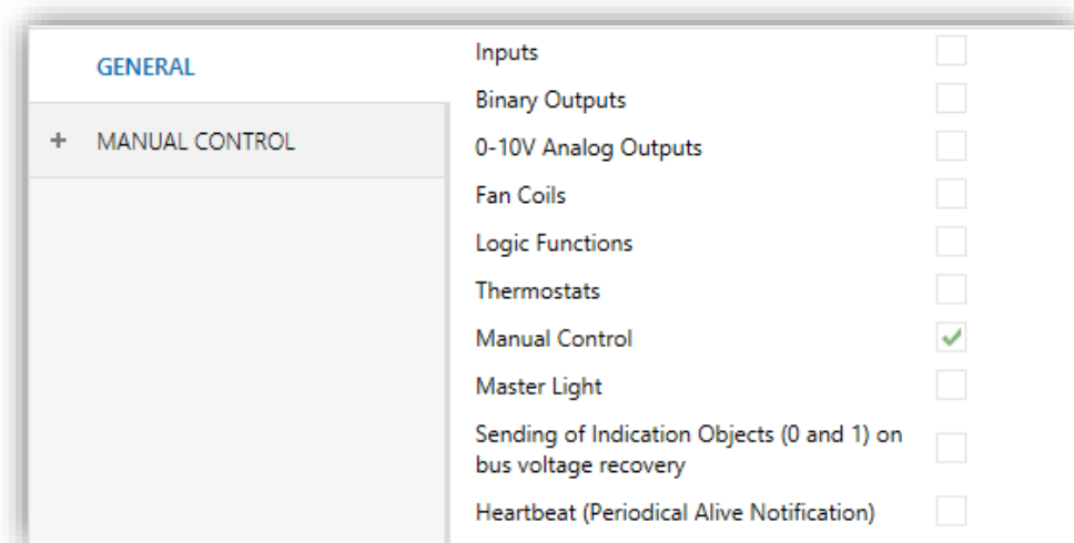
Figure 2 General screen.
