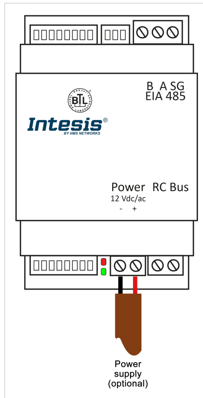
Figure 2. Power connector
