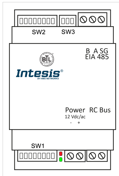
Figure 4. IN485HIT001R000 DIP switches
