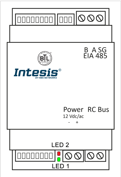
Figure 5. IN485HIT001R000 LEDs
