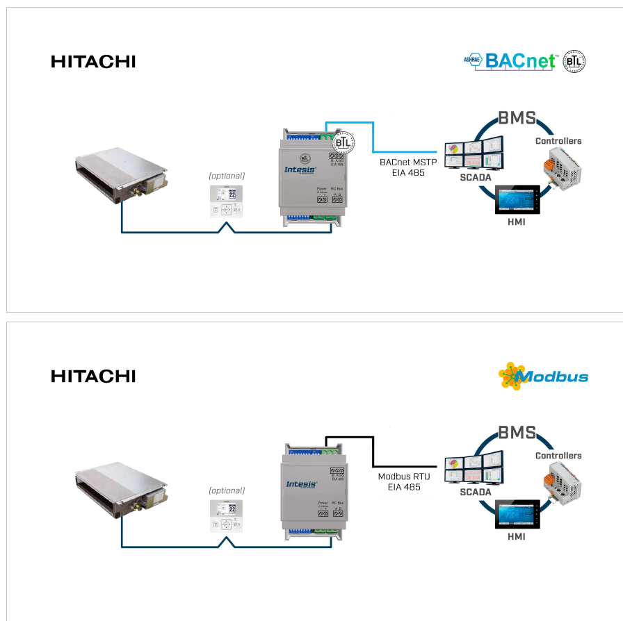
Figure 1. Integration of Hitachi AC units into a BACnet or Modbus installation using the Intesis IN485HIT001R000 gateway
