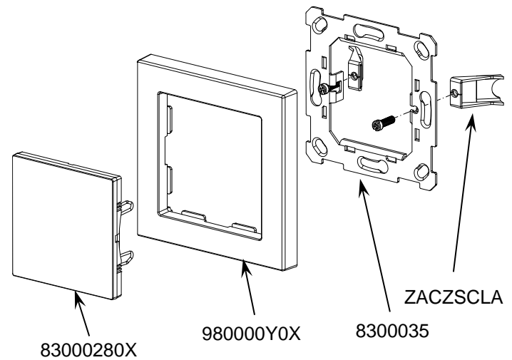
Figure 1. Blind panel.
