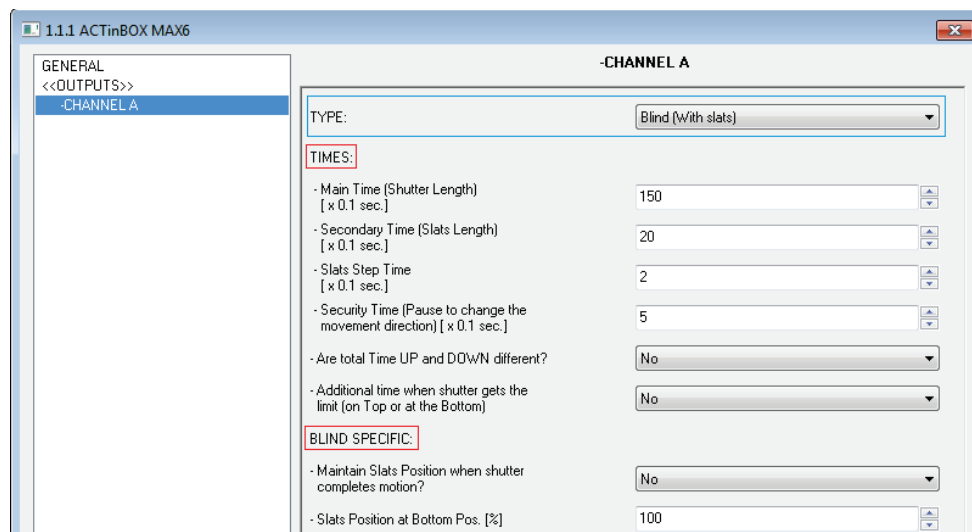
Figure 21 Blinds with slats. Configuration screen (ETS)
