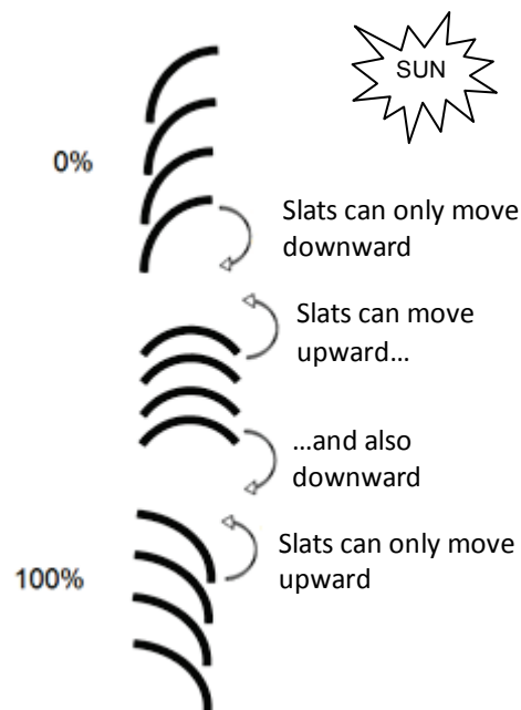
Figure 20 Slat positions
