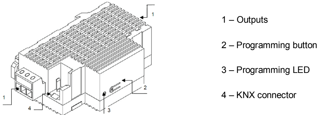
Figure 2 ACTinBOX MAX6. Element Scheme
