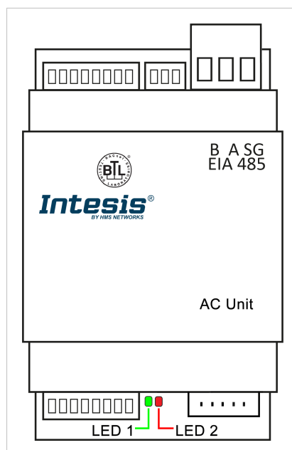
Figure 3. IN485DAI001I000 LEDs
