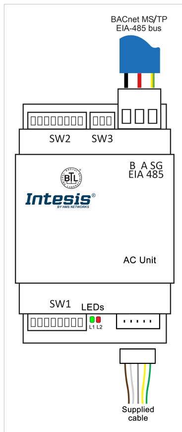
Figure 2. Wiring diagram (wire colors are indicative only. The AC unit cable may have four or five poles)
