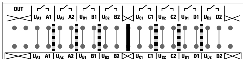
Fig. 4 Insulation properties of the clamp groups ■■■ Insulation 6 kV (increased insulation) ■■■ Insulation 4 kV (single insulation)
