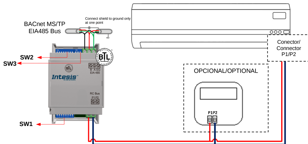
Figure 2.2 Connection diagram
